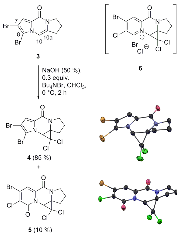
Scheme 1. Cyclopropanation of dipyrrolopyrazinone 3 . Yields of 4 and 5 change to 35 % each after 12 h. Molecular structures of 4 [3] and 5 in the crystal (displacement ellipsoids at the 50 % probability level, hydrogen atoms omitted for clarity).
