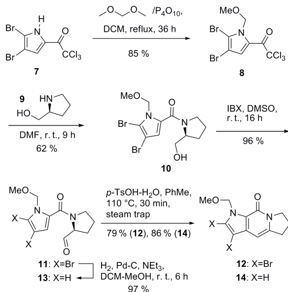
Scheme 2. Synthesis of dipyrrolopyridinones 12 and 14 with inverted pyrrole rings.
